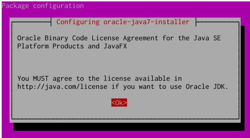
Figura 7.6: Java installer
